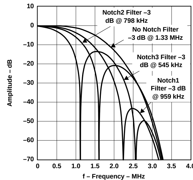
Figure 2–9. Color Low-Pass Filter With Notch Filter Frequency Response (PAL Square Pixel Sampling)
