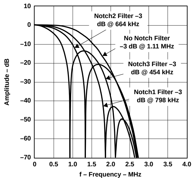
Figure 2–7. Color Low-Pass Filter With Notch Filter Frequency Response (NTSC And PAL-M Square Pixel Sampling)
