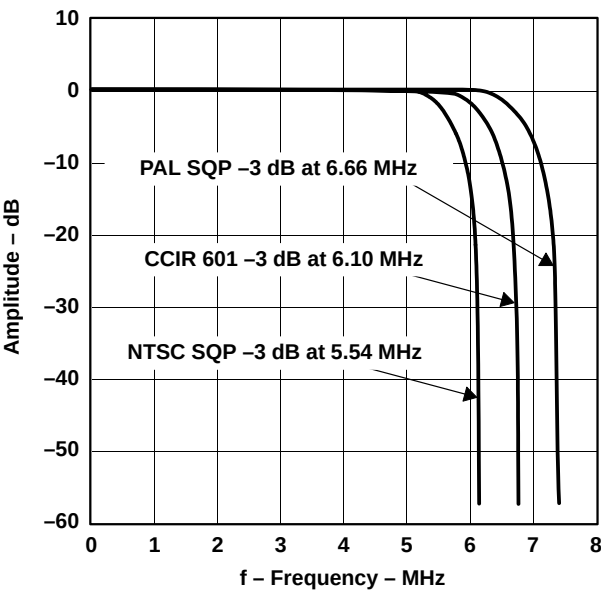
Figure 2–4. Decimation Filter Frequency Response
